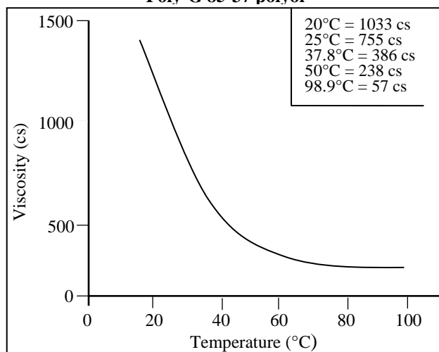
Figure 1 Viscosity vs. Temperature Poly-G 85-37 polyol
