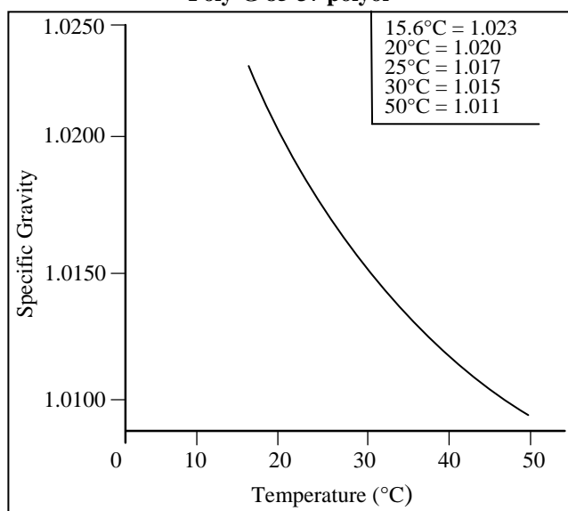
Figure 2 Specific Gravity vs. Temperature Poly-G 85-37 polyol
