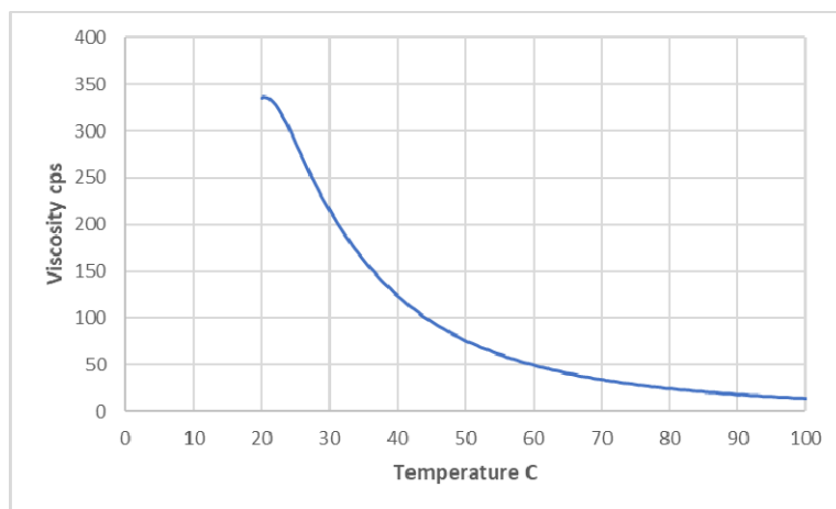
Figure 1 Viscosity vs. Temperature Poly-G 85-240 polyol
