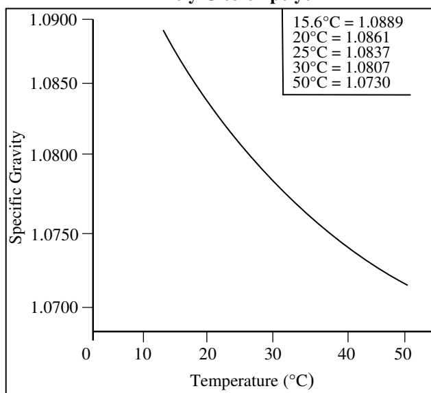
Figure 2 Specific Gravity vs. Temperature Poly-G 83-34 polyol
