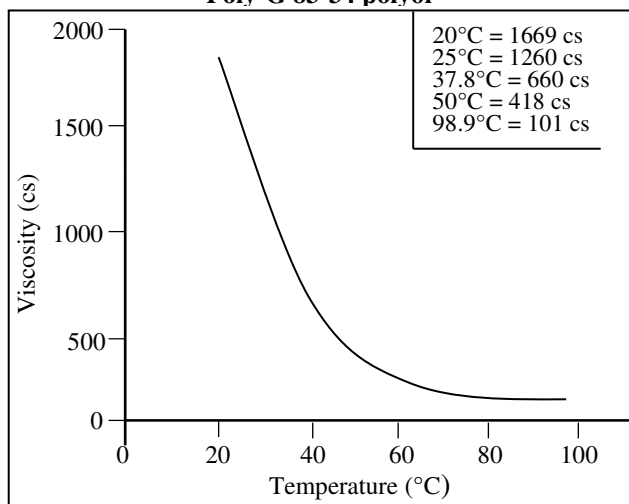
Figure 1 Viscosity vs. Temperature Poly-G 83-34 polyol
