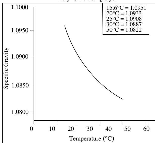
Figure 2 Specific Gravity vs. Temperature Poly-G 76-635 polyol
