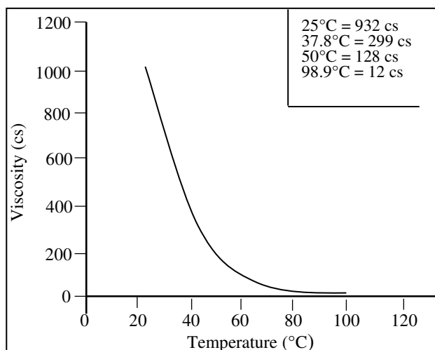
Figure 1 Viscosity vs. Temperature Poly-G 76-635 polyol
