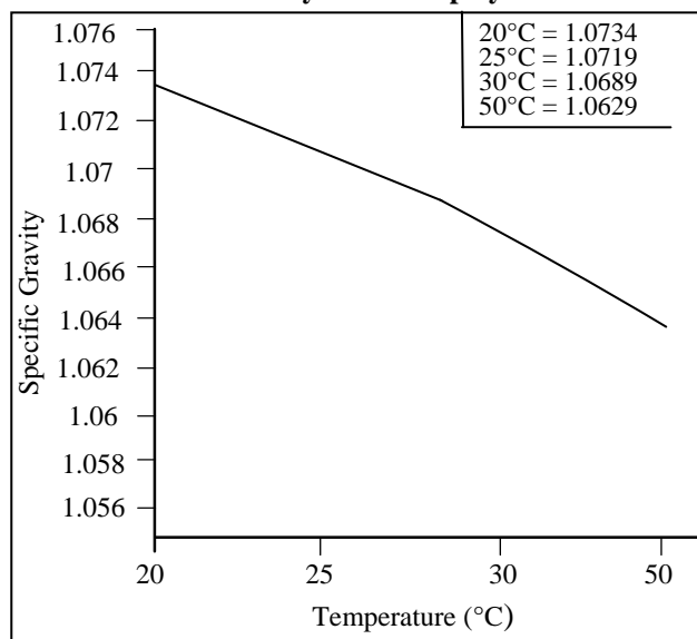
Figure 2 Specific Gravity vs. Temperature Poly-G 71-357 polyol
