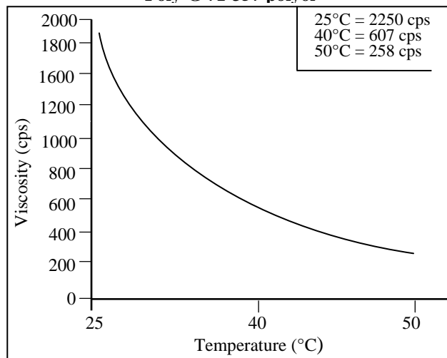
Figure 1 Viscosity vs. Temperature Poly-G 71-357 polyol
