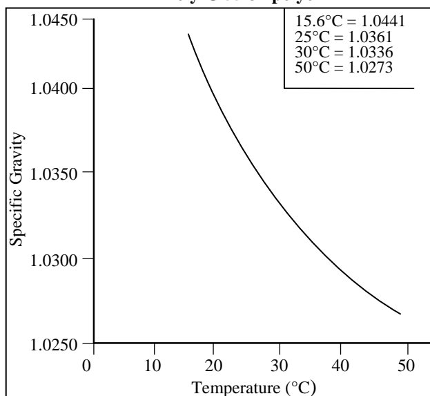
Figure 2 Specific Gravity vs. Temperature Poly-G 55-37 polyol
