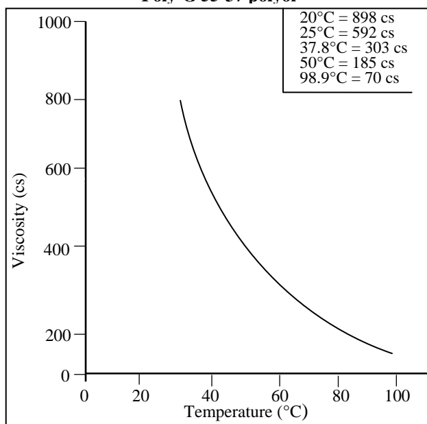
Figure 1 Viscosity vs. Temperature Poly-G 55-37 polyol
