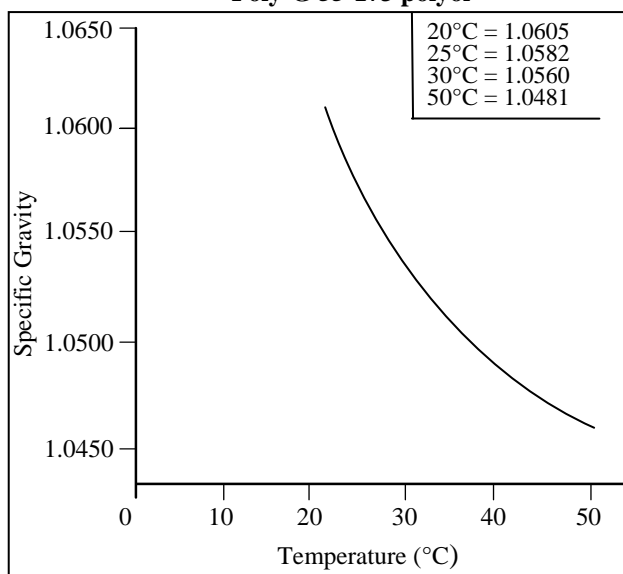
Figure 2 Specific Gravity vs. Temperature Poly-G 55-173 polyol
