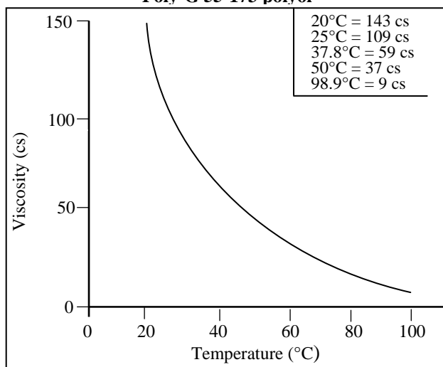
Figure 1 Viscosity vs. Temperature Poly-G 55-173 polyol
