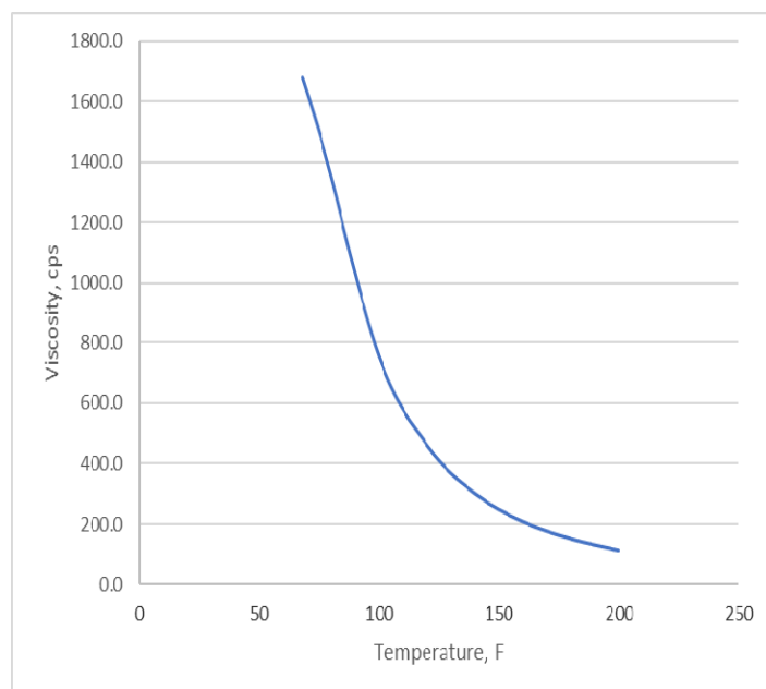
Figure 1 Viscosity vs. Temperature Poly-Q 53-35
