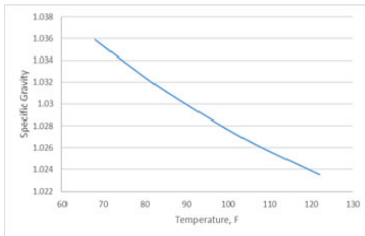
Figure 2 Specific Gravity vs. Temperature Poly-Q 53-35
