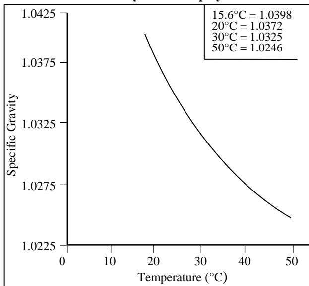
Figure 2 Specific Gravity vs. Temperature Poly-G 30-280 polyol
