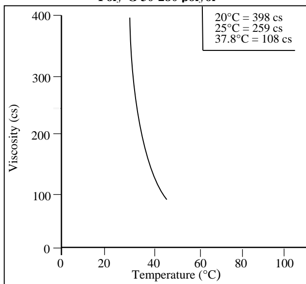
Figure 1 Viscosity vs. Temperature Poly-G 30-280 polyol
