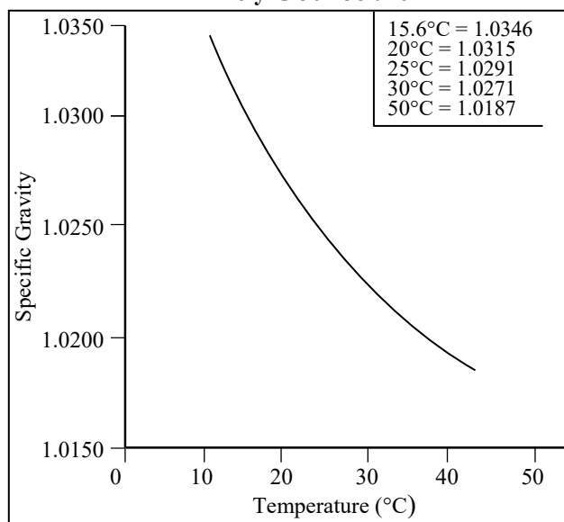
Figure 2 Specific Gravity vs. Temperature Poly-G 30-238 triol
