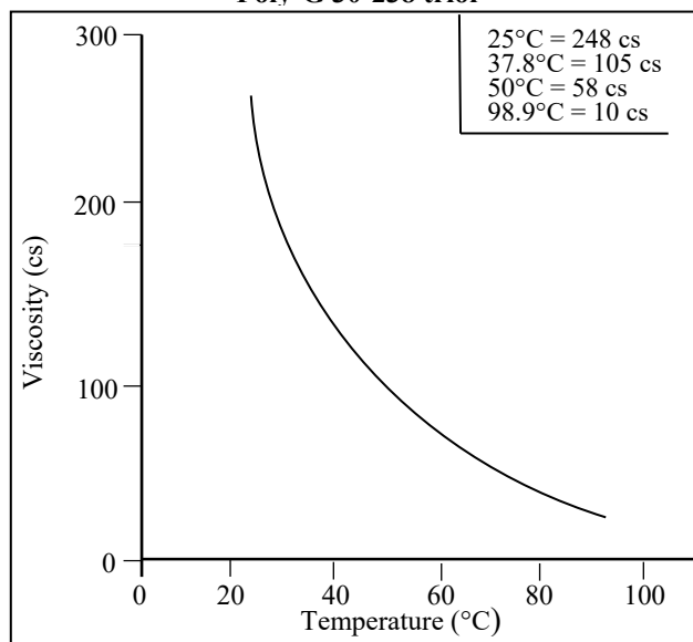
Figure 1 Viscosity vs. Temperature Poly-G 30-238 triol
