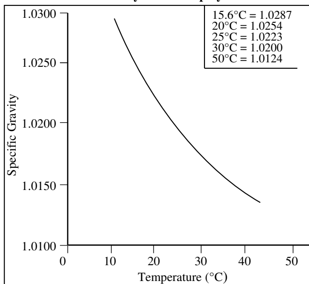
Figure 2 Specific Gravity vs. Temperature Poly-G 30-169 polyol
