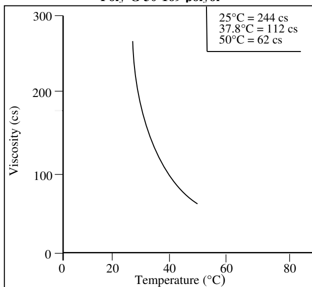
Figure 1 Viscosity vs. Temperature Poly-G 30-169 polyol
