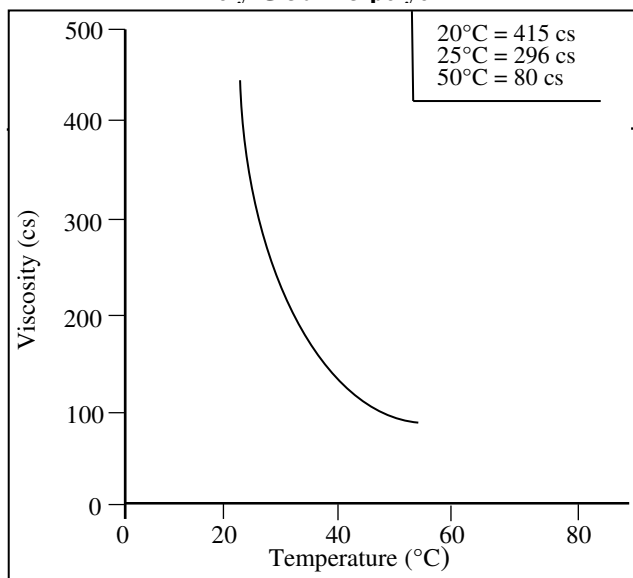
Figure 1 Viscosity vs. Temperature Poly-G 30-113 polyol
