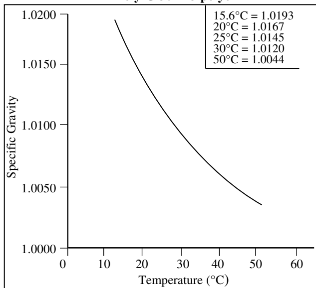
Figure 2 Specific Gravity vs. Temperature Poly-G 30-113 polyol
