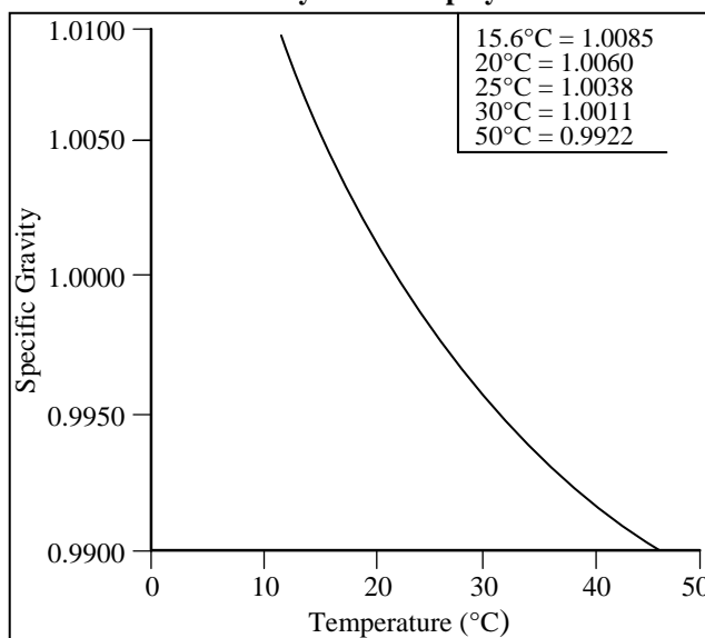
Figure 2 Specific Gravity vs. Temperature Poly-G 26-150 polyol
