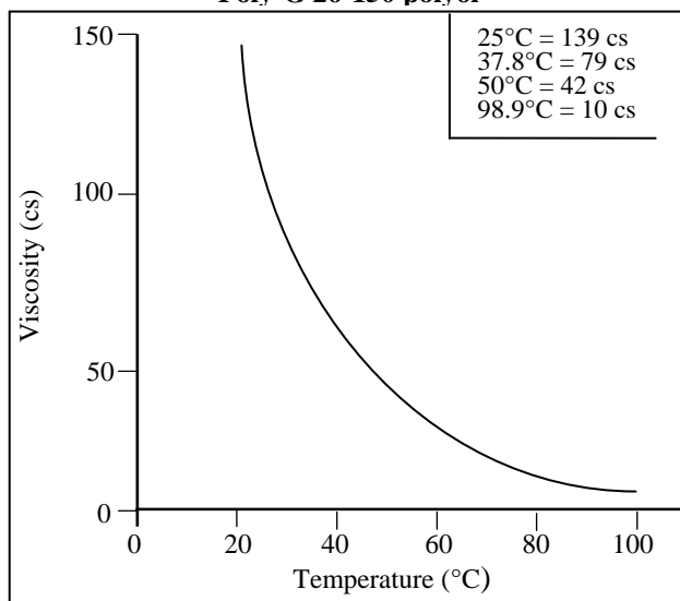
Figure 1 Viscosity vs. Temperature Poly-G 26-150 polyol
