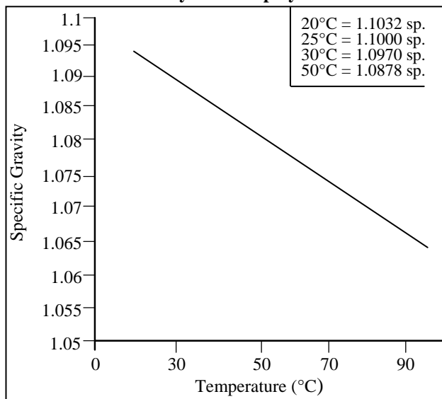
Figure 2 Specific Gravity vs. Temperature Poly-G 22-56 polyol
