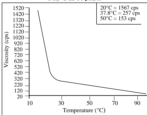
Figure 1 Viscosity vs. Temperature Poly-G 22-56 polyol
