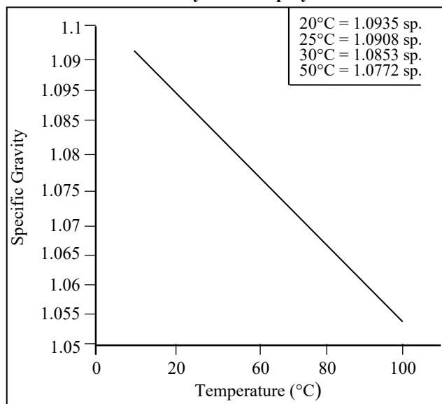
Figure 2 Specific Gravity vs. Temperature Poly-G 22-37 polyol
