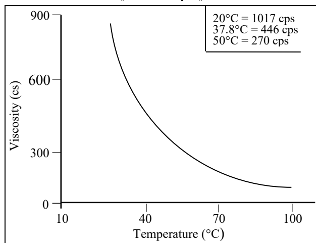
Figure 1 Viscosity vs. Temperature Poly-G 22-37 polyol
