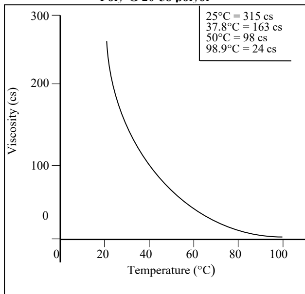
Figure 1 Viscosity vs. Temperature Poly-G 20-58 polyol
