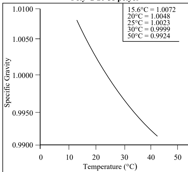
Figure 2 Specific Gravity vs. Temperature Poly-G 20-58 polyol
