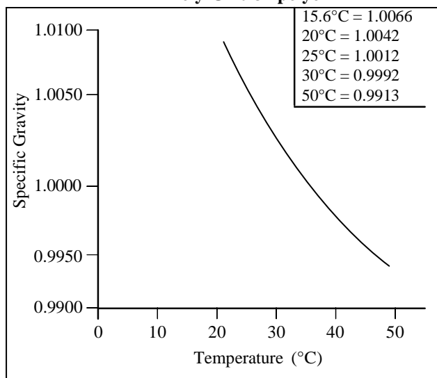
Figure 2 Specific Gravity vs. Temperature Poly-G 20-37 polyol
