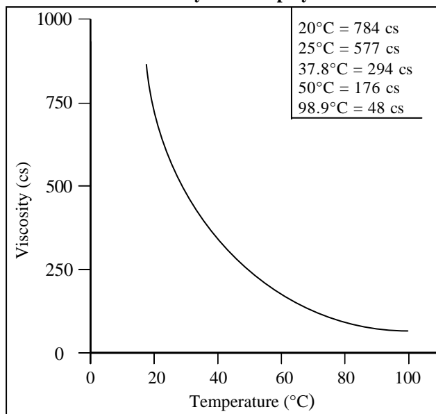
Figure 1 Viscosity vs. Temperature Poly-G 20-37 polyol
