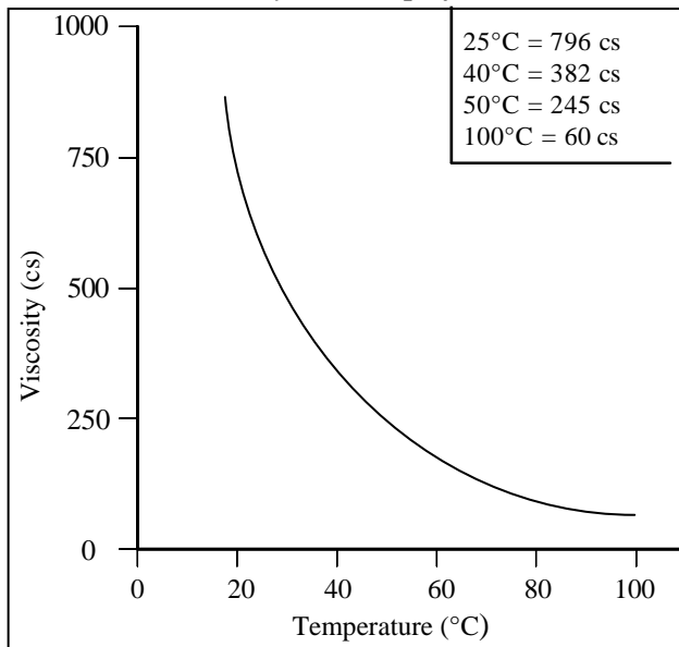
Figure 1 Viscosity vs. Temperature Poly-G 20-28 polyol
