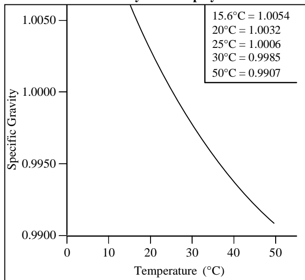
Figure 2 Specific Gravity vs. Temperature Poly-G 20-28 polyol
