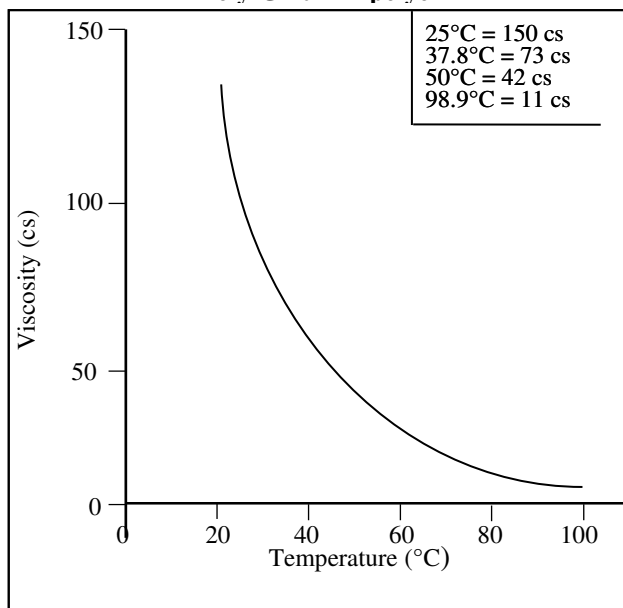
Figure 1 Viscosity vs. Temperature Poly-G 20-112 polyol
