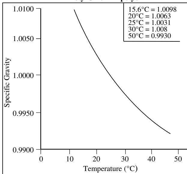
Figure 2 Specific Gravity vs. Temperature Poly-G 20-112 polyol
